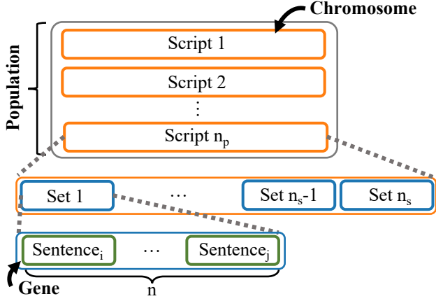
Fig. 3. GA terms and their corresponding definitions. The population is a collection of scripts, each chromosome is a script, each gene is a sentence, and n_p , n_s , and n denote the number of scripts in the population, number of sets in a script, and number of sentences in a set, respectively. Sentence i denotes the i -th sentences in the candidate sentence set. The sentences were randomly sampled from the candidate sentence set during initialization, and there were no duplicate sentences in each script.
