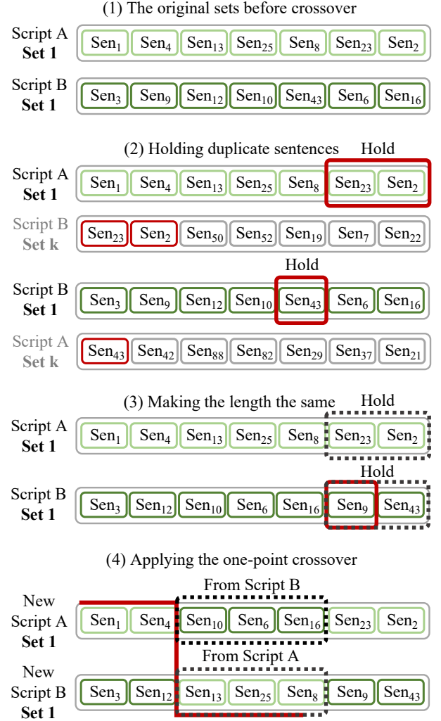
Fig. 7. (1) The original sets before crossover. Sen i denotes the i -th sentence in the candidate sentence set. (2) Holding duplicate sentences. In this example, Sen 23 and Sen 2 are held because they exist in a set in Script B. Similarly, Sen 43 is held because it already exists a set in Script A. These sentences are not exchanged during the crossover process to avoid duplicate sentences in the script. If Sen 23 and Sen 2 are exchanged to Script B, there will be two Sen 23 and two Sen 2 in Script B. (3) Making the length the same. Because the number of duplicate sentences in Set 1 of Script A and Set 1 of Script B are not the same (i.e., two sentences in Set 1 of Script A and one sentence in Set 1 of Script B), we randomly hold one more sentence (Sen 9 ) in Set 1 of Script B. (4) Applying the one-point crossover.
