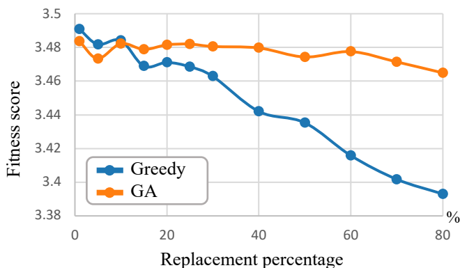
Fig. 11. Comparison between the GA- and greedy-based replacement methods in the postprocessing phase. The greedy-based method outperforms the GA-based method when the replacement percentage is lower than 10%; however, as the replacement percentage increases, the GA-based method outperforms the greedy-based method.
