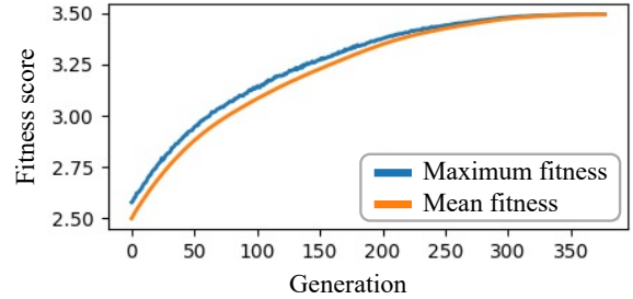
Fig. 9. Training curve of the GA. Overall, the fitness score increases with the number of generations and then eventually converges.
