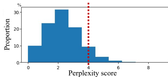
Fig. 8. Perplexity distribution for ten-character sentences in Mandarin Chinese news texts. The red dotted line represents the threshold used for the perplexity filter.
