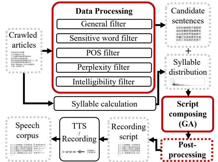
Fig. 1. Schematic diagram of the proposed BASPRO system. In the data processing phase, candidate sentences were extracted from the collected articles. The script-composing phase uses real-world syllable distribution to compose a syllable-balanced script from the candidate sentences. Finally, the postprocessing phase replaces unwanted sentences in the script and produces the final script.
