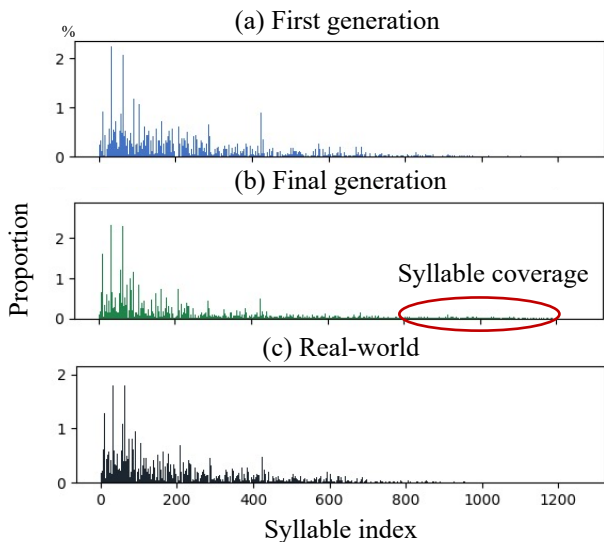
Fig. 10. Distribution of syllables in the best scripts of the first and final generations and in real-world texts. The results show that the best script in the final generation has a syllable distribution that is closer to real-world syllable distribution than the best script in the first generation. The red region reveals the effect of script_syllable_coverage ; that is, more rare syllables are covered in the best script in the final generation.
