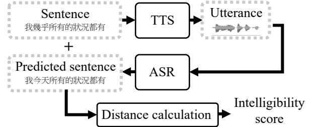
Fig. 2. Illustration of the intelligibility score calculation. First, a sentence is converted into an utterance using a TTS system. Then, an ASR system is used to predict the content of the utterance. The distance between the sentence and ASR prediction is used to calculate the intelligibility score.
