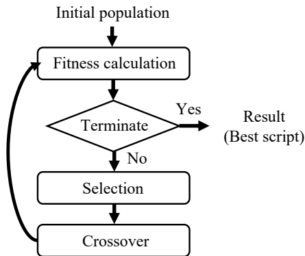
Fig. 4. Schematic diagram of GA. The termination condition occurs when the maximum fitness score no longer increases after several generations.
