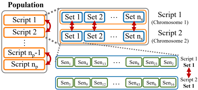
Fig. 6. Illustration of the crossover pairs. The crossover step exchanges sentences between two sets with the same index.
