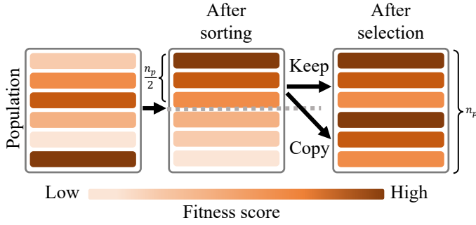
Fig. 5. Illustration of the truncation-selection process. The scripts are sorted by their fitness scores, and then 50% of the fittest scripts are selected and replicated twice.
