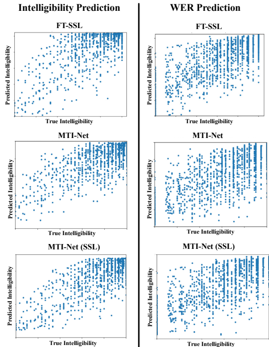
Figure 2: Scatterplots of three speech intelligibility prediction models, including FT-SSL [14], MTI-Net, and MTI-Net(FT-SSL).
