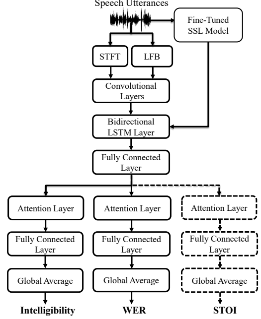
Figure 1: Architecture of the MTI-Net model.
