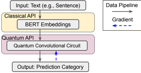
Fig. 1: BERT-QTC for vertical federated [11] text classification.
