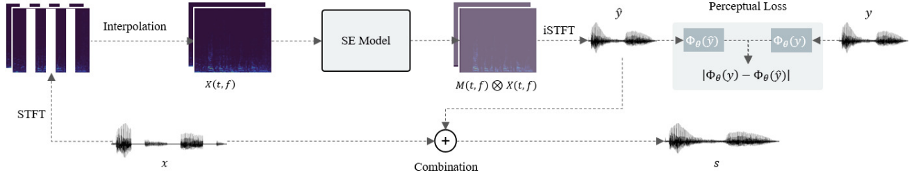
Fig. 1. System architecture of the proposed ISR system.
