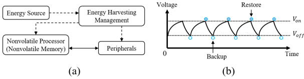
Fig. 2. (a) self-powered intermittent system (b) general voltage trace of self-powered intermittent systems [11]
