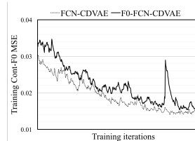
Figure 5: Training Cont-F0 MSE of the F0 prediction network.
