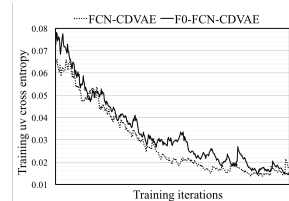
Figure 6: Training uv cross entropy of the F0 prediction network.
