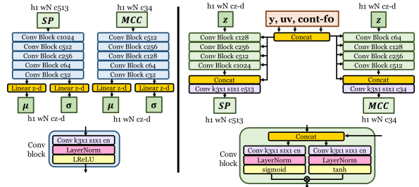
Figure 4: Model architecture. The input is of length N . h , w , c means height, width and channels. z - d means latent code dimension. LReLU, LayerNorm means leaky rectified activation function and layer normalization layer. k , s , c means kernel size, stride and output channels.
