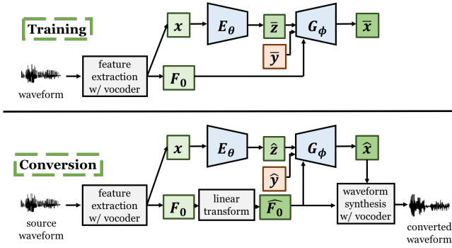
Figure 3: The proposed framework with F_0 conditioning.
