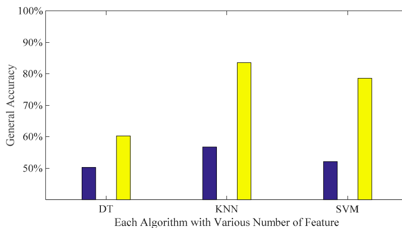
Figure 10. Comparison between two different numbers of features on vehicle mode detection accuracy of three machine learning algorithms.
