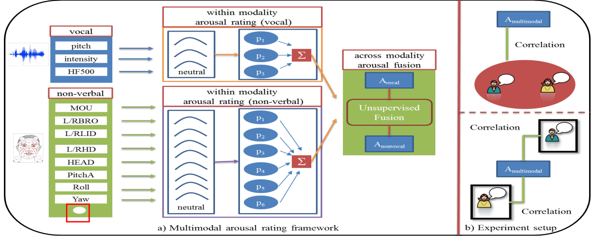
Fig. 2. a) A work flow on computing arousal by fusing intra- (within) and inter- (cross) modalities. b) A depiction on the evaluation setup of experiment I, II and experiment III, where experiment I assess the correlation of the framework with the average human raters, and experiment III assesses the correlation between the framework and individual raters
